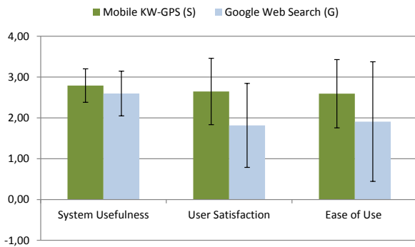
Figure 4. Average number of points (within a 7-point Likert scale) of the system usefulness, user satisfaction, and ease of use, with error bars indicating standard deviation around the mean.
