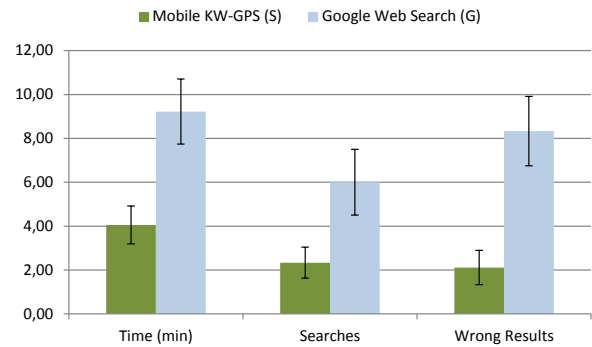
Figure 5. Statistical data collected during the user evaluation about the time users spent to complete the task, number of searches, and number of wrong results.
