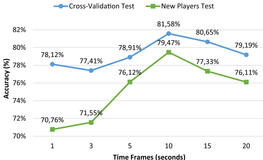
Fig. 11. Average accuracy of the proposed model for different time frames (cross-validation test and new players test).
