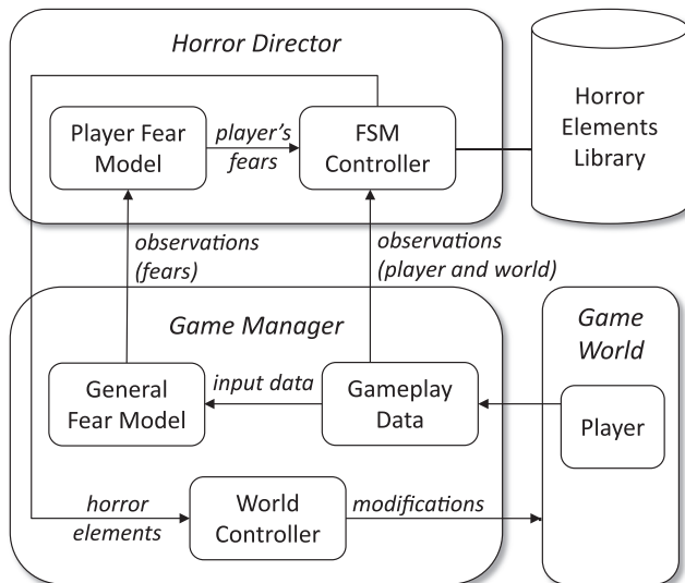
Fig. 7. Architecture of the adaptive horror game system.
