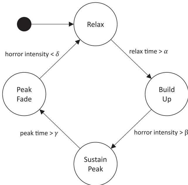
Fig. 8. Finite State Machine of the Horror Director .
