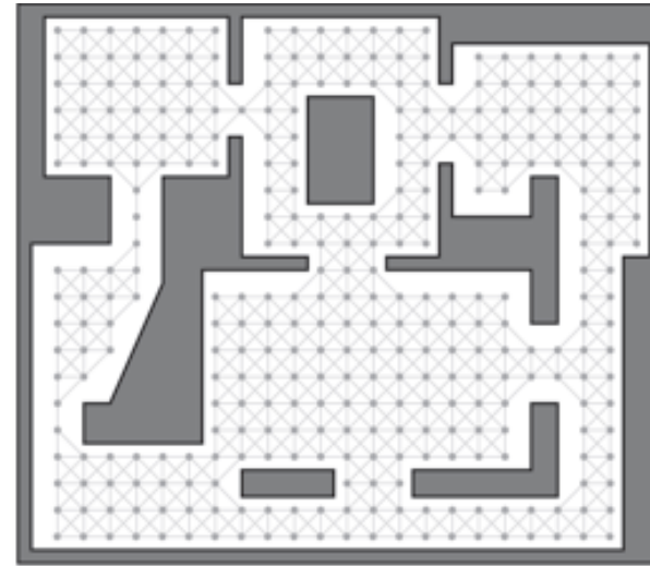
Low-Level Graph
