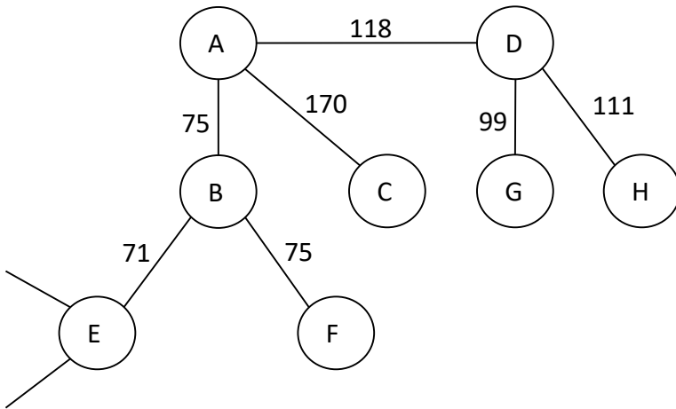
Graph:
