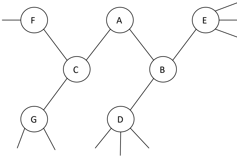
Graph:
