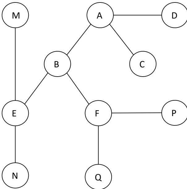
Graph:
