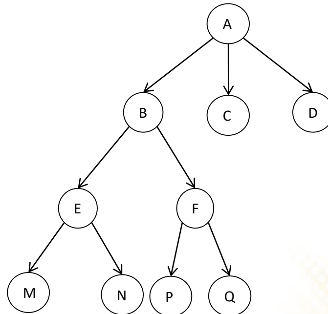
Search Tree:
