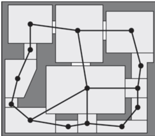
High-Level Graph
