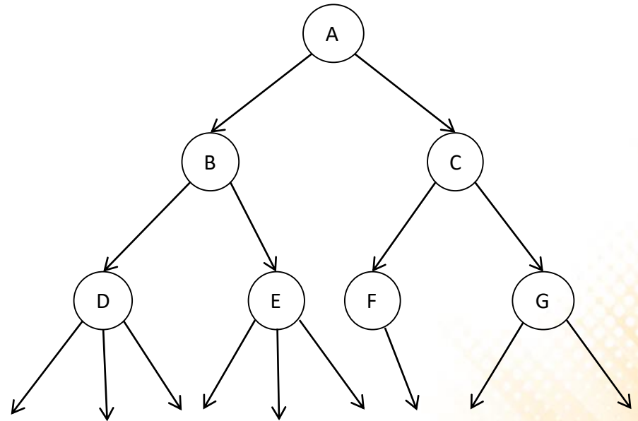
Search Tree:
