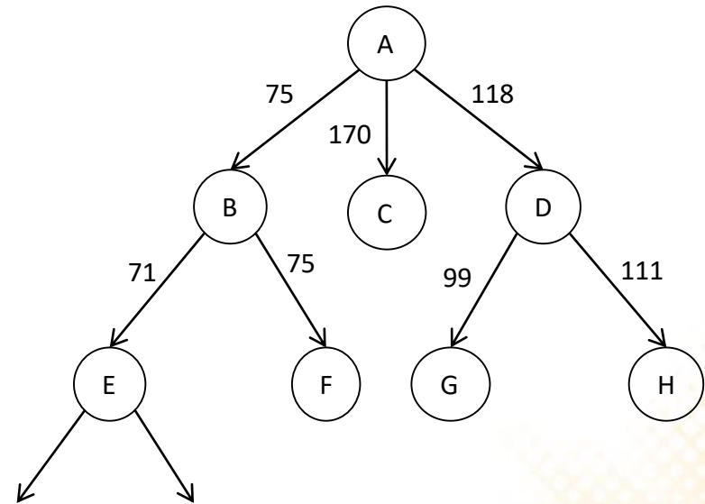
Search Tree:
