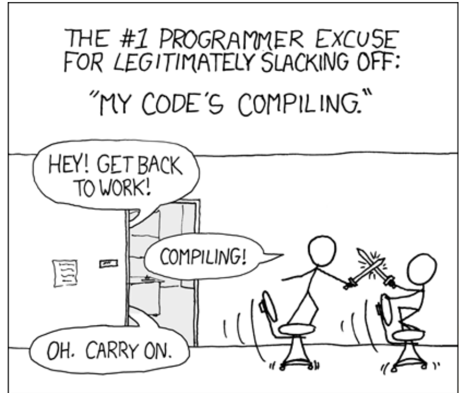
Executable code
